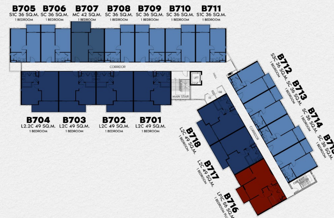
7 TH FLOOR
